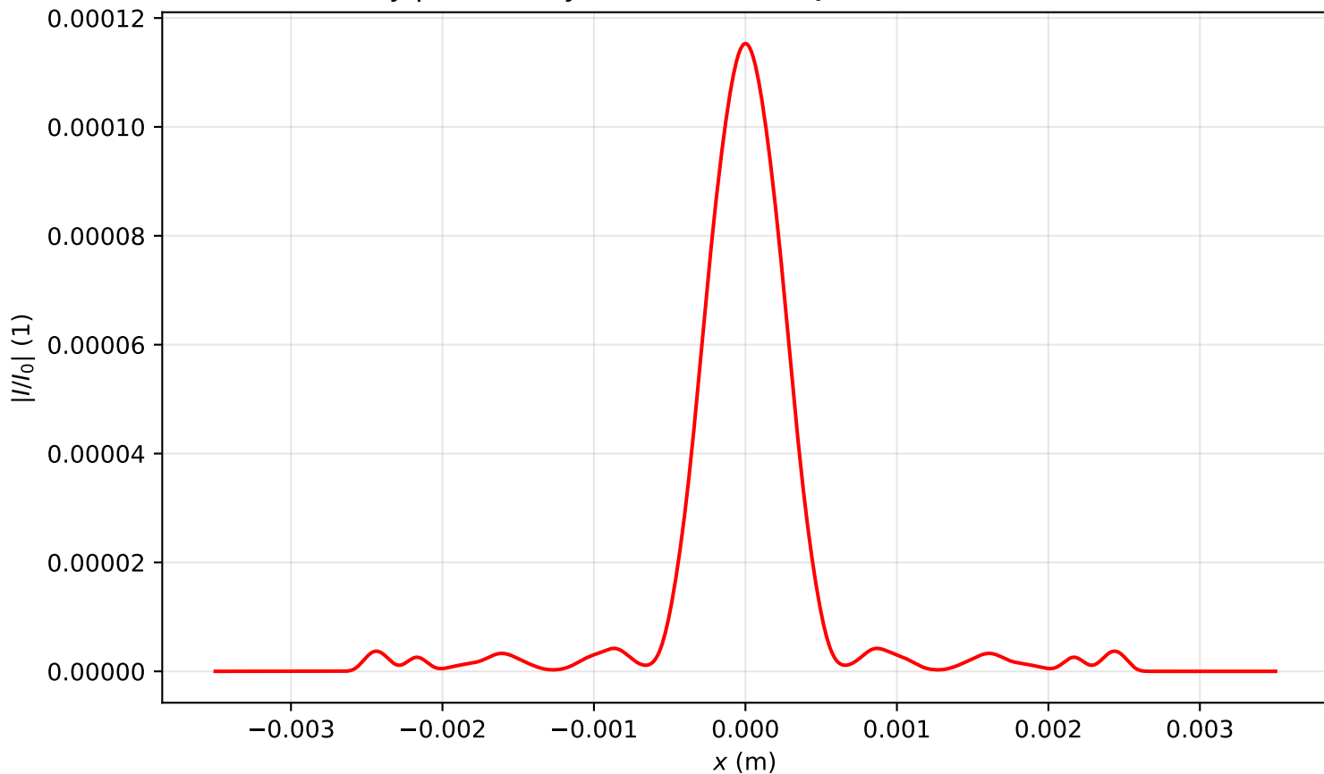
Intensity profile I(x, y = 0, z = 1.831)/I_0 , P_{in}=9.0P_{cr} , artificial time
